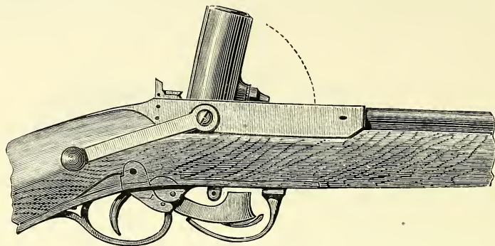
Norwegian Carbine: 1842 Model.
